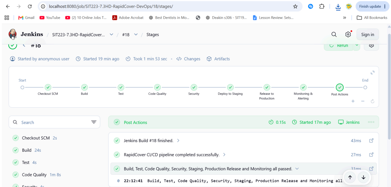
Figure 1: Jenkins Build #18 successfully completing the full RapidCover CI/CD pipeline from build and testing through security, staging, production release and monitoring.
