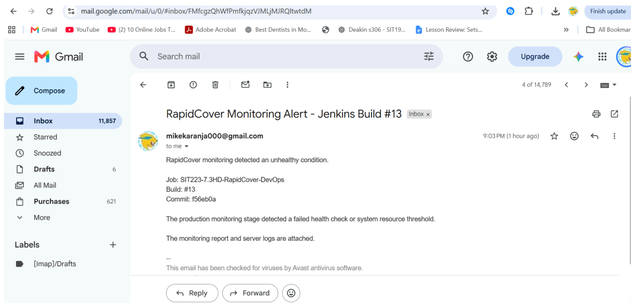
Figure 6: Automated monitoring alert generated during Build #13 when an unhealthy condition was detected, demonstrating the pipeline's failure-alert path.
