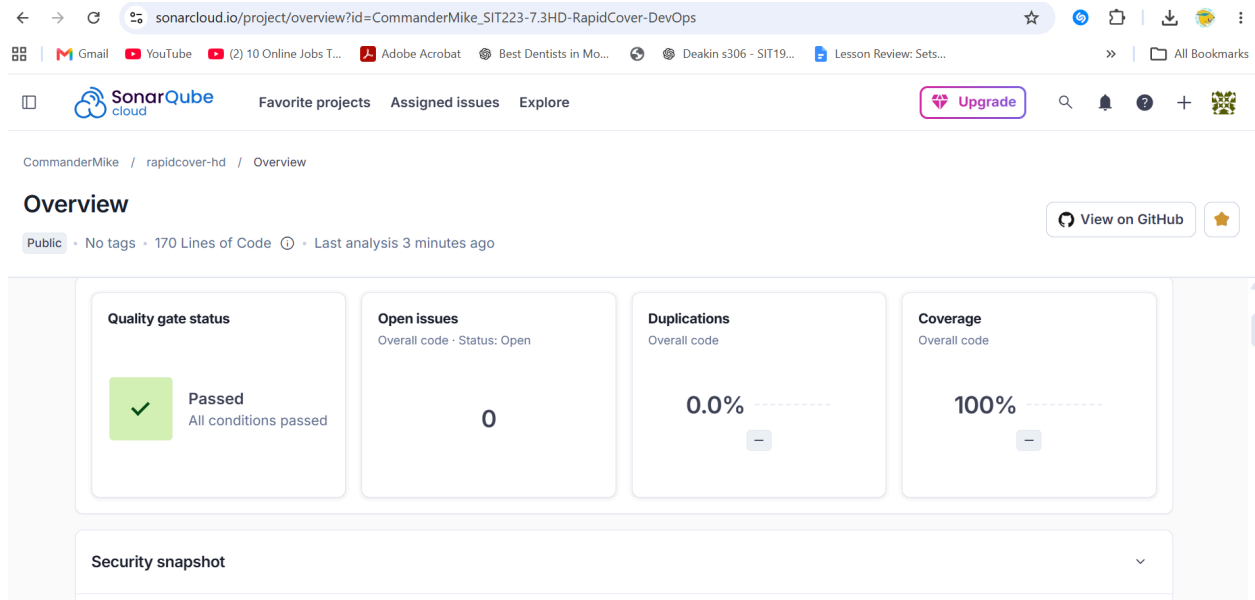
Figure 3: SonarQube Cloud quality gate passing with 100% coverage, zero open issues and zero duplication.
